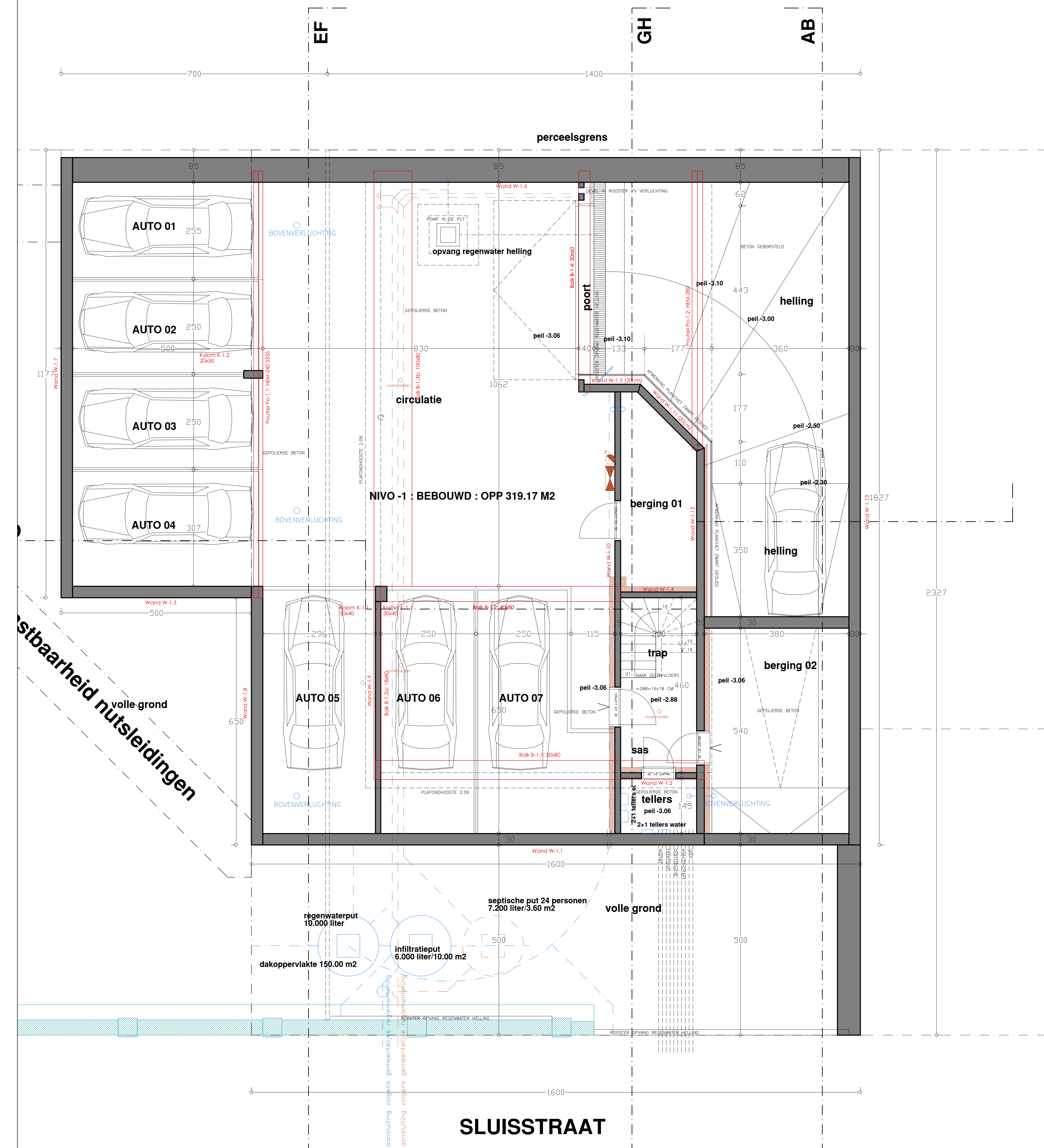
KELDER -1
